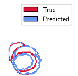
segmentations
